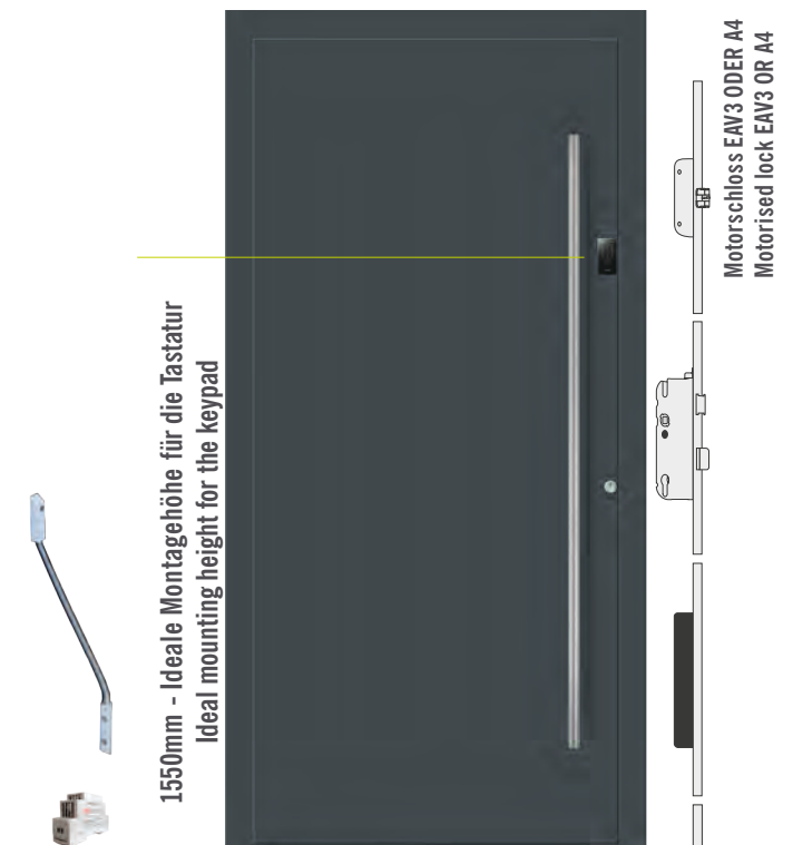
white keypad WKB - 48x94mm
